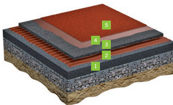
1 Asphalt or concrete layer on gravel bed • 2 Adhesive • 3 Regupol® elastic layer • 4 Sealed pores of the Regupol® elastic layer • 5 PUR-EPDM wear layer
