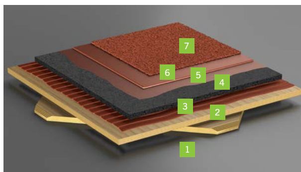
1 Sub surface (e.g. screed) • 2 Wood panel • 3 Adhesive layer 4 Regupol® base mat • 5 PU pore sealer • 6 Self levelling PU layer (wear coat) • 7 EPDM granules (wear coat)
