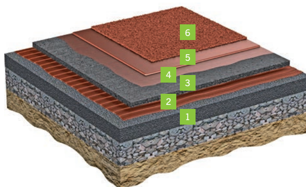
1 Asphalt layer on gravel bed • 2 PUR adhesive • 3 Regupol® elastic layer, prefabricated • 4 Sealed pores of the Regupol® elastic layer • 5 Cast layer made of PUR • 6 Wear layer made of EPDM granules
