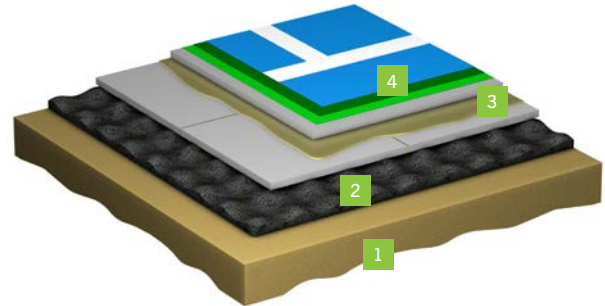
1 Unbound base • 2 Regupol® elastic layer with dimpled surface • 3 2 layers of light-weight concrete sheets, laminated • 4 Wearing surface in 3 layers: Special primer (bright green ), filler coat (dark green), top coating with games lines (blue)
